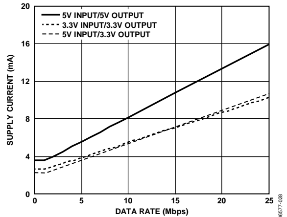
Figure 21. Typical I_{CH} Supply Current per Forward Data Channel (15 pF Output Load)
