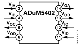
Figure 3. ADuM5402
