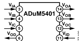
Figure 2. ADuM5401
