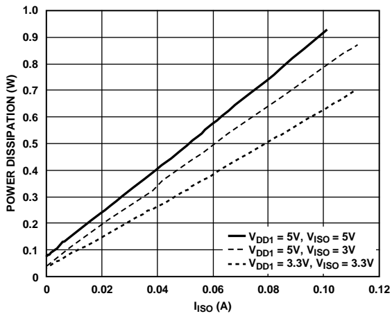
Figure 12. Typical Total Power Dissipation vs. Isolated Output Supply Current in All Supported Power Configurations
