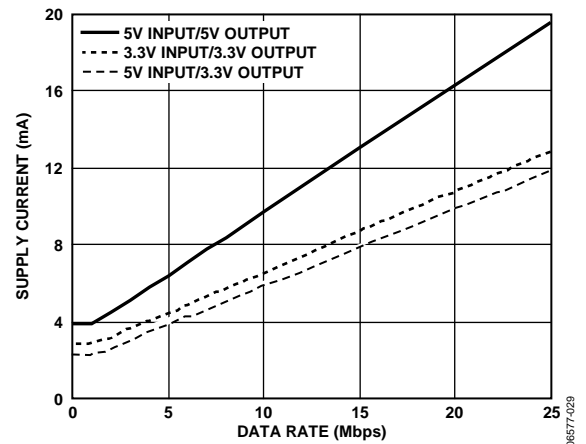
Figure 22. Typical I_{CH} Supply Current per Reverse Data Channel (15 pF Output Load)
