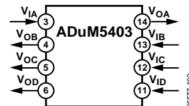
Figure 4. ADuM5403
